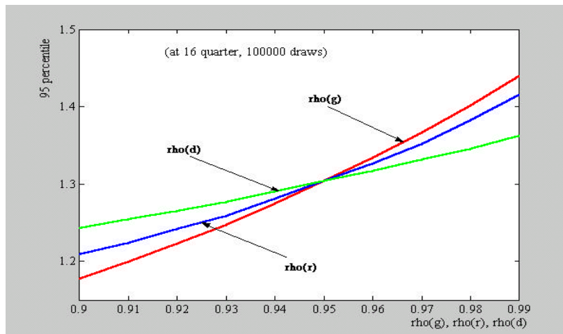
Figure 6: Sensitivity of the 95 th percentile of b to changes in the autoregressive parameters.
